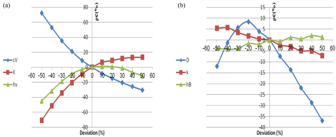
Fig. 2. a. Percentage change in \rho_c(\%) with deviation (%) from original parameter value ( c_v , K , h_v ). Figure 2b. Percentage change in \rho_c(\%) with deviation (%) from original parameter value ( D , k , h_B )
