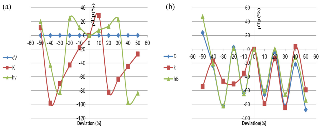
Fig. 3. . a. Percentage change in \rho_{Tp}(\%) with deviation (%) from original parameter value ( c_v , K , h_v ). Figure 3b. Percentage change in \rho_{Tp}(\%) with deviation (%) from original parameter value ( D , k , h_B )
