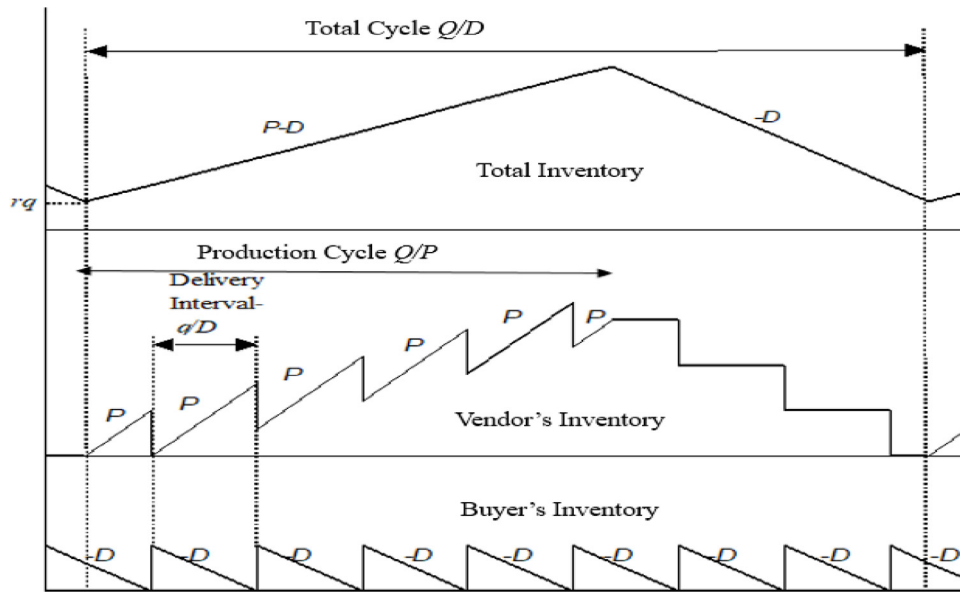
Fig. 1. Inventory level at the buyer, inventory level at the manufacturer, and total inventory (adapted from David, I., & Eben-Chaime, M., 2008)
