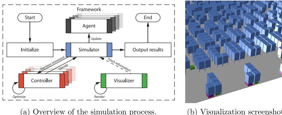
Fig. A1. RAWSim-O simulation framework.
