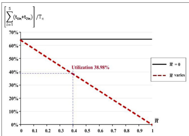
Fig. 8. The effect of deviations in \bar{\pi} on sum of machine utilization.
