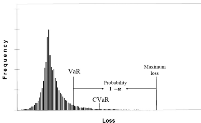
Fig. 1. VaR and CVaR [22].
