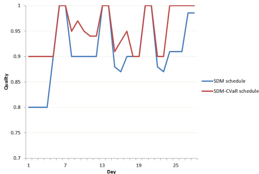
Fig. 2. Quality factors of SDM and SDM-CVaR schedule.
