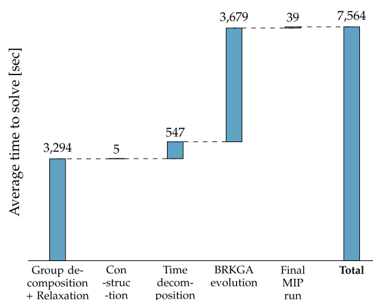
Fig. 11. Average time to solve each each component of the proposed method.
