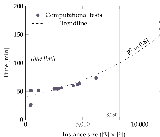
Fig. 5. Time to generate group decomposition and relaxation initial prices, using (M)INLP models.
