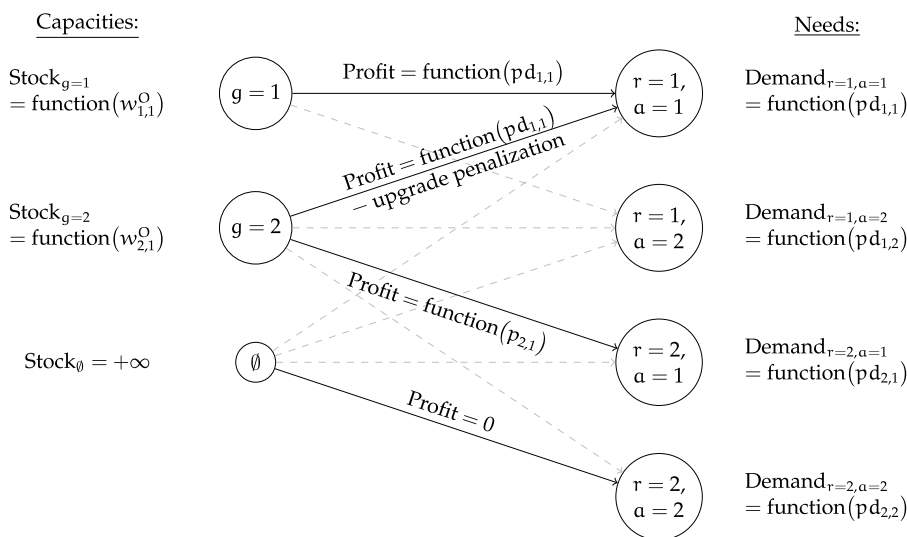
Fig. 14. Representation as a “transportation” problem, with capacities on the origin nodes (stock of vehicle groups) and needs on the destination nodes (demand for related rental types): zoom in a specific location ( s = 1 ) and time ( t = 1 ). The notation follows the mathematical model notation presented in Section 2.2.1 and, for
