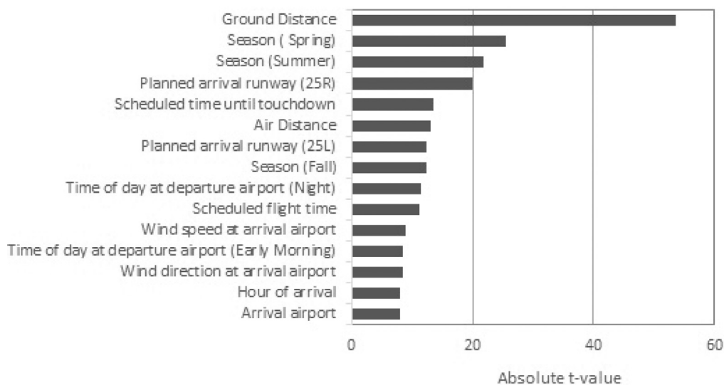
Fig. 9. Variable importance plot: Linear regression including all variables. Absolute t-value as measurement. Not fully comparable to linear regression in the ensemble model due to variable selection and different ensemble stages.
