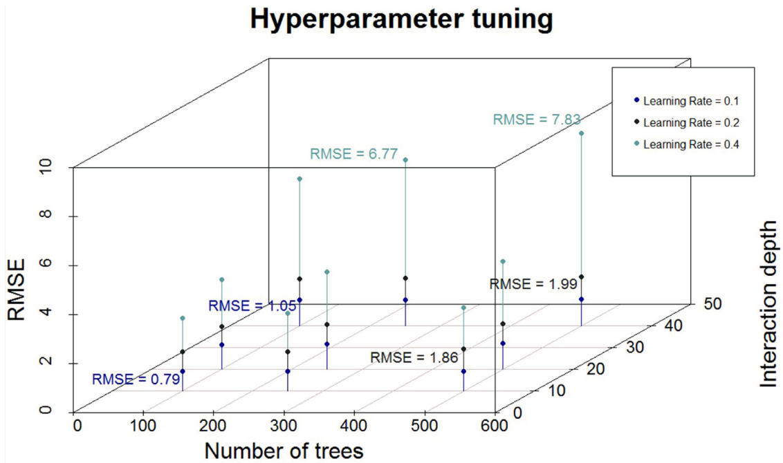
Fig. 5. Increasing interaction depth leads to a slight increase in RMSE. Overall a low learning rate delivers superior results. The effect of number of trees on RMSE depends on learning rate and interaction depth.
