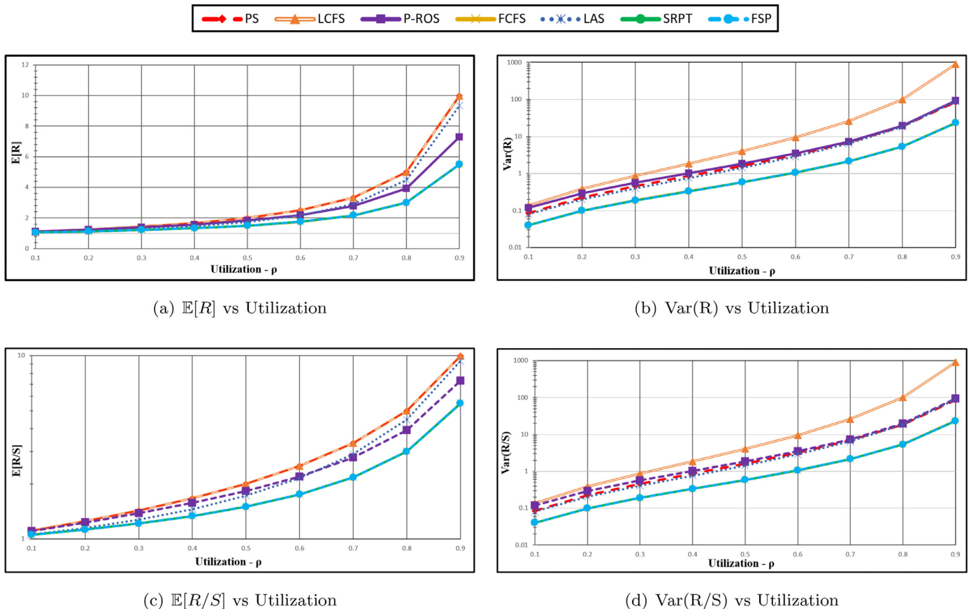
Fig. 3. Simulation results for system where service times are constant: a = 1 .
