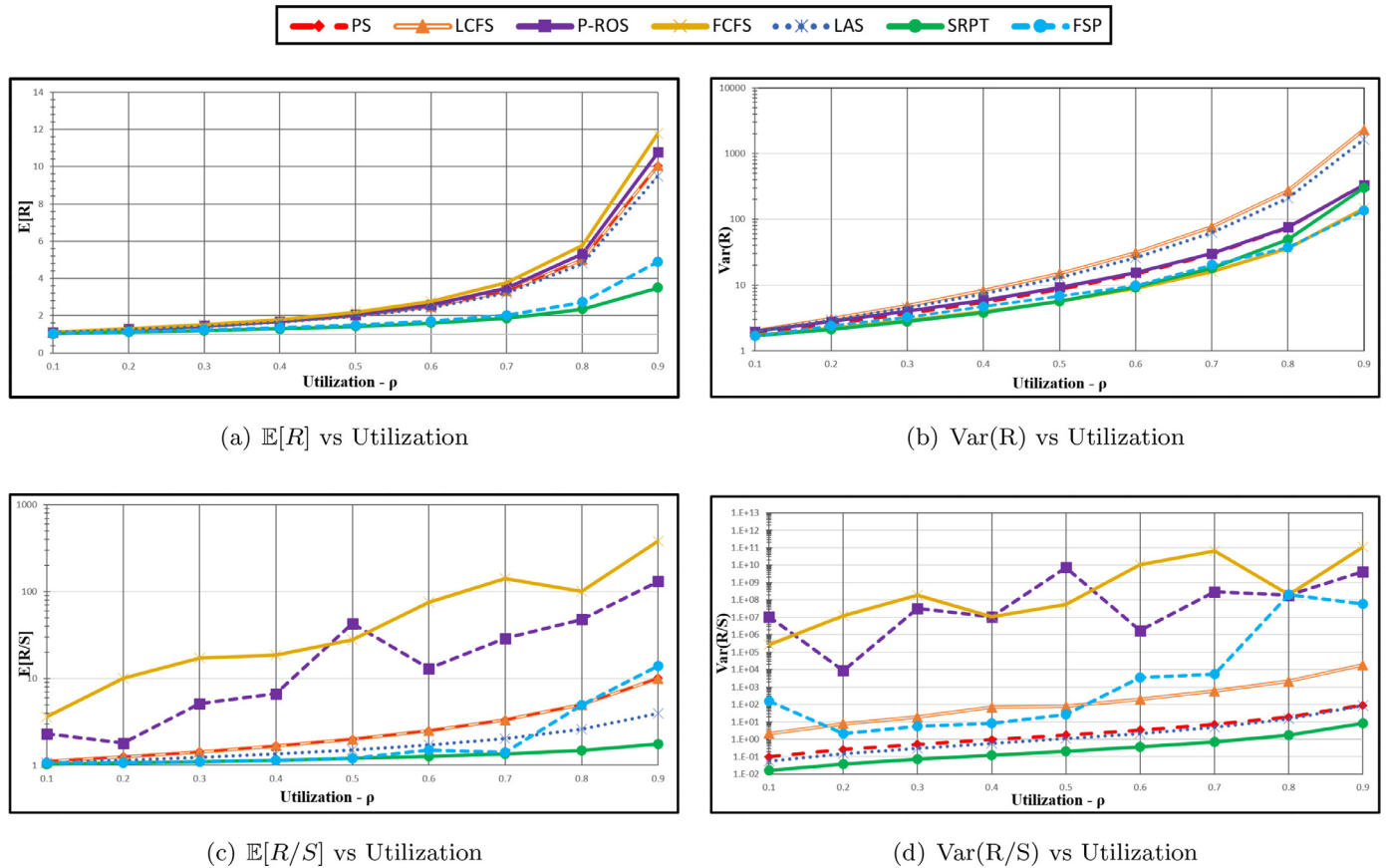
Fig. 10. Numerical results for systems where service times follow a hyper-exponential distribution: p_1 = 0.75, p_2 = 0.25, 1/\mu_1 = 1.25, 1/\mu_2 = 0.25 , where p_i denotes the probability of sampling from an exponential distribution with corresponding rate \mu_i .
