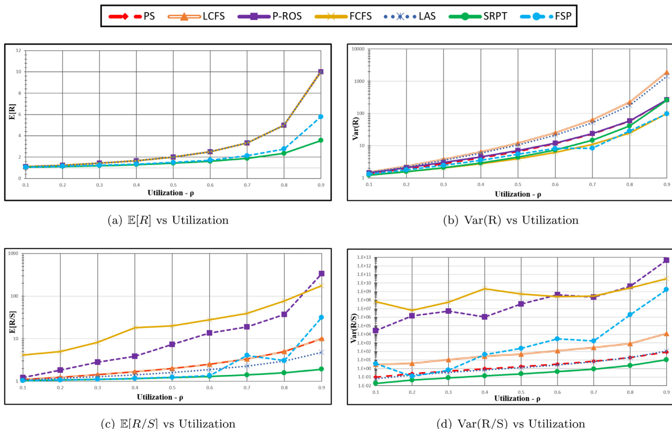
Fig. 8. Simulation results for systems where service times are exponentially distributed: 1/\mu = 1 .
