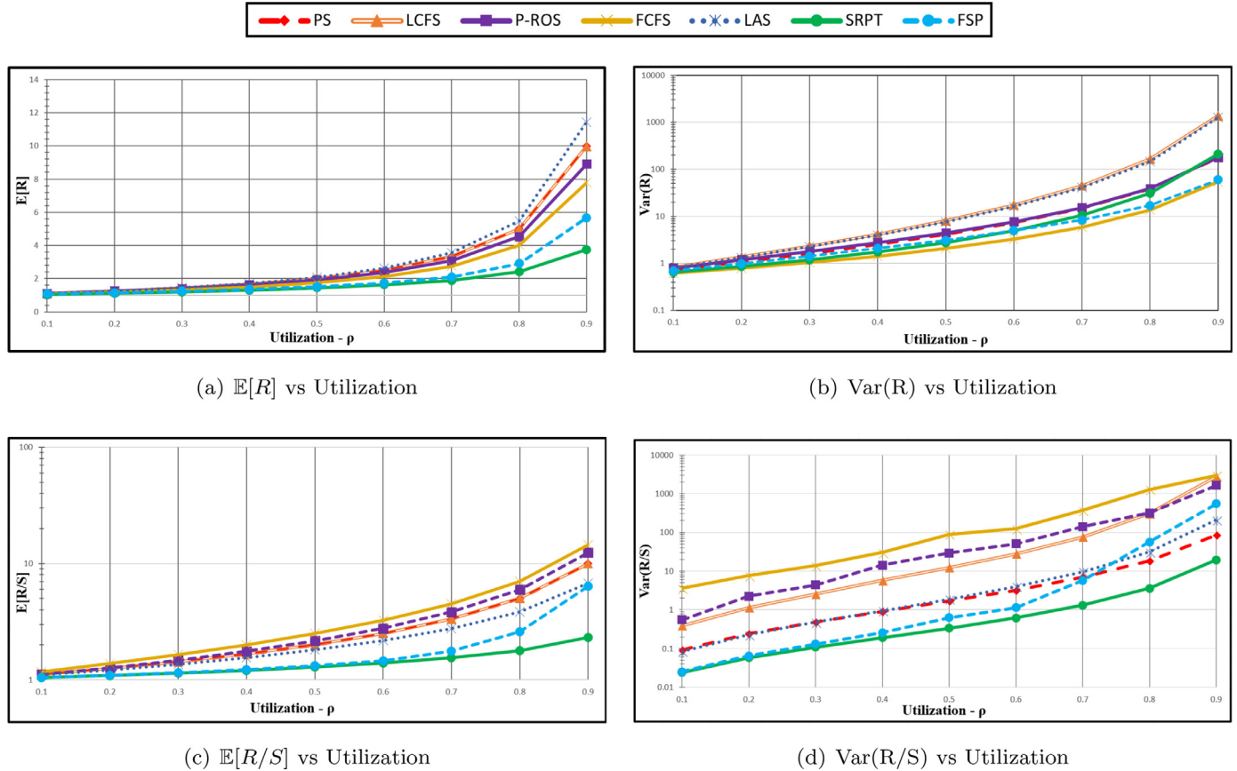
Fig. 4. Simulation results for systems where service times follow an Erlang distribution: k = 2, 1/\mu = 0.5 .
