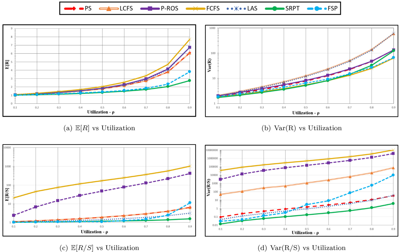
Fig. 6. Simulation results for systems where service times follow a bounded hyper-exponential distribution; p_1 = 0.75 , p_2 = 0.25 , 1/\mu_1 = 1.24 , 1/\mu_2 = 0.24 , and lower bound of 0.01, where p_i denotes the probability of sampling from an exponential distribution with corresponding rate \mu_i .
