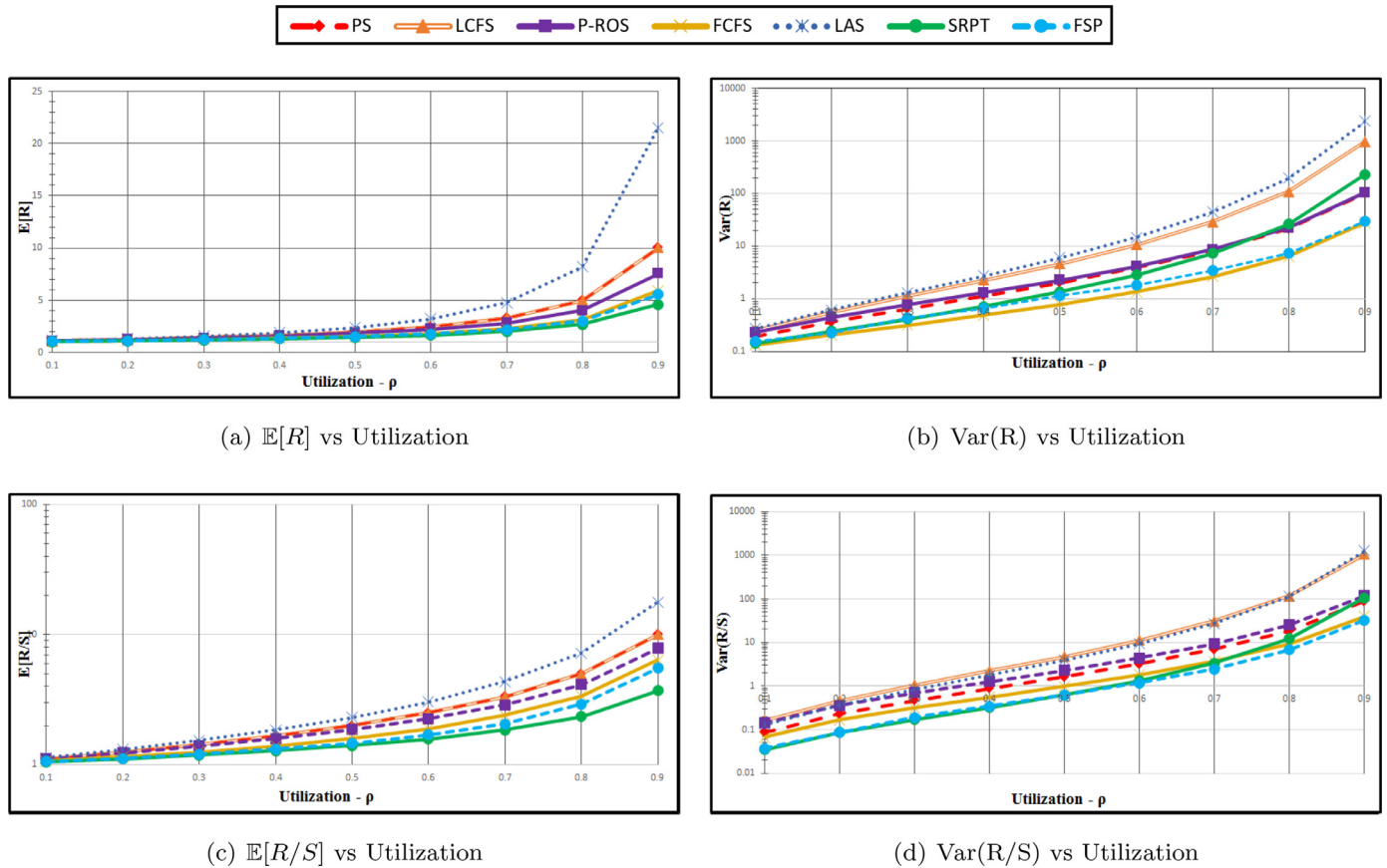
Fig. 5. Simulation results for systems where service times follow a uniform distribution: a = 0.5, b = 1.5 .
