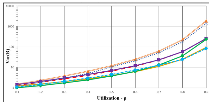
(b) \text{Var}(R) vs Utilization
