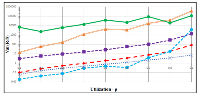
(c) \text{Var}(R/S) vs Utilization
