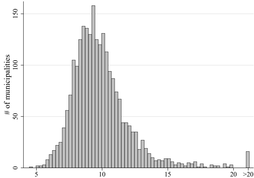
Notes: Histogram depicts the distribution of the ratio between the 90 th and the 10 th income percentile at the municipal level ( N = 2,360 ) for the year 2003.
