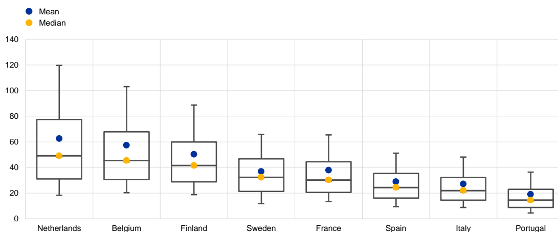
TFP level distribution in selected EU countries, 2010
