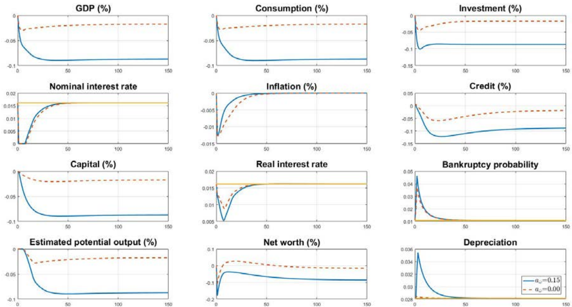
Figure 7: Baseline simulation vs case without disruption spillovers
