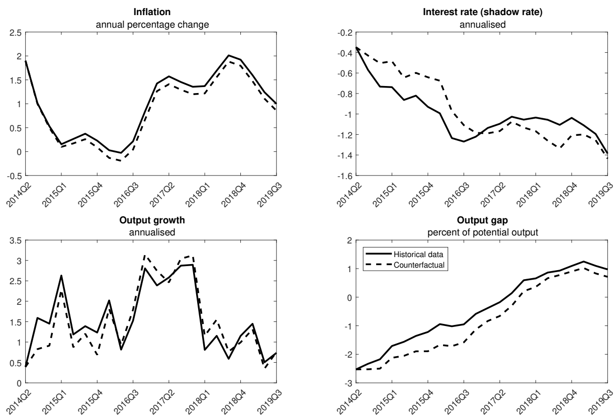
Figure 4: Counterfactual exercise
