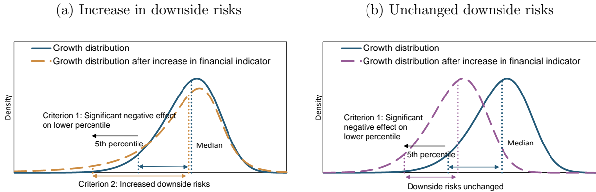
Figure 1: Illustration of growth-at-risk and downside risks to growth using distribution of GDP growth.
