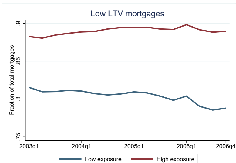
Figure C.1: LTV-persistence
