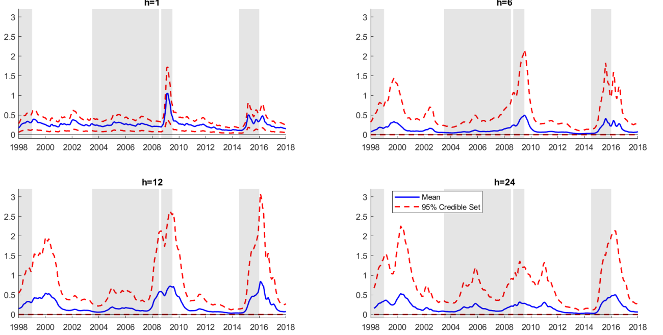
Figure 13: Means of the MVH ratios, including 95% credibility regions, over the forecast evaluation period.
