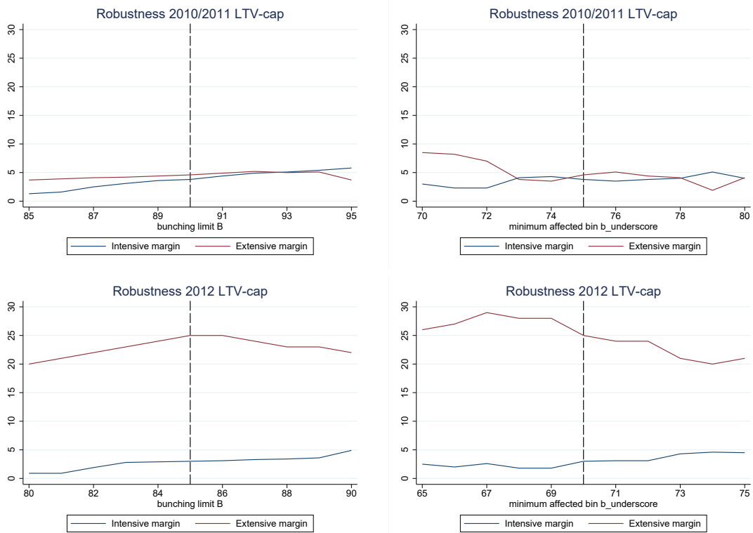
Figure A6: Sensitivity of bunching analysis to changing \underline{b} and B for 2010/2011 requirement and 2012 requirement.
