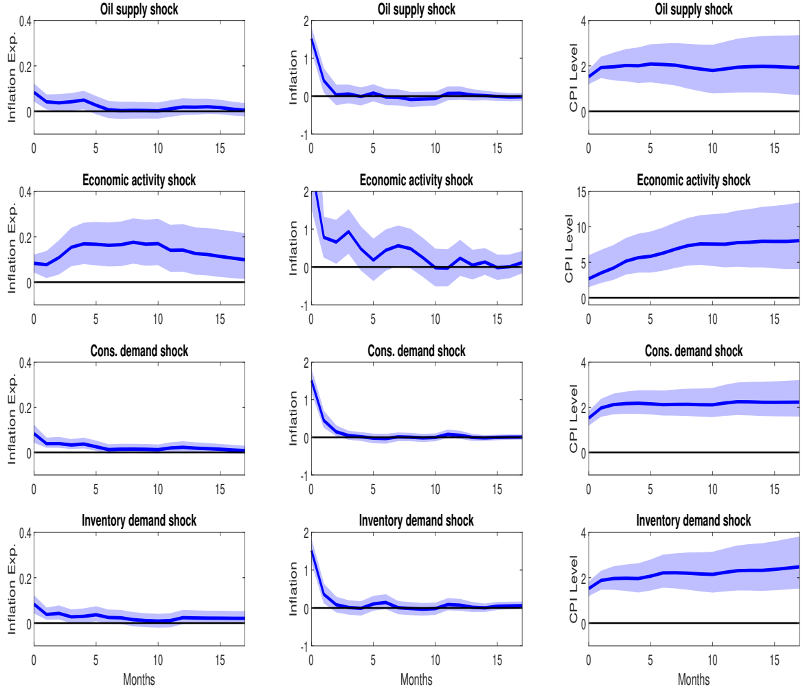
Figure 2: Structural impulse response functions
