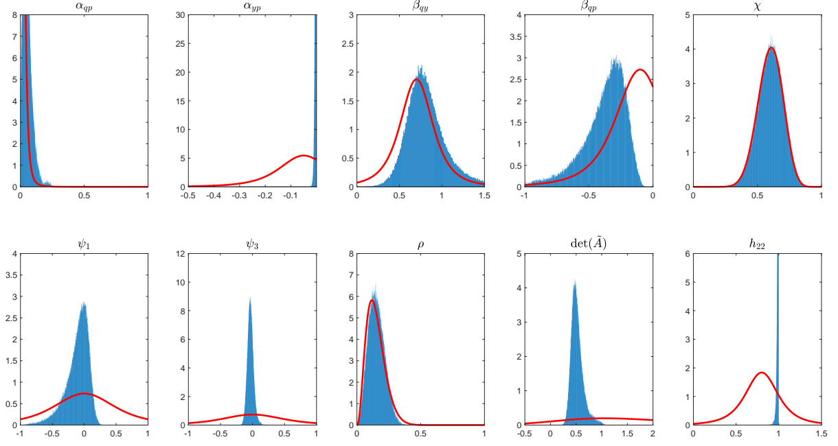
Figure 10: Prior (solid red curves) and posterior (blue histograms) distributions of structural parameters in the oil block
