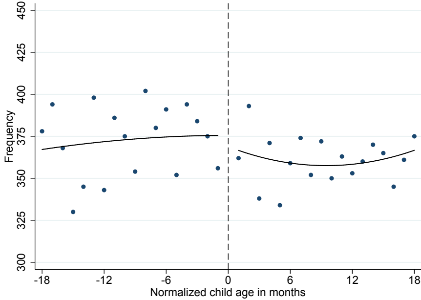
FIGURE 3: DENSITY AROUND THRESHOLD
