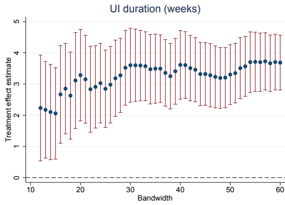
(c) 1 st -order polynomial
