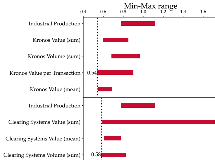
Figure 14: Root mean squared error for GDP nowcasting
