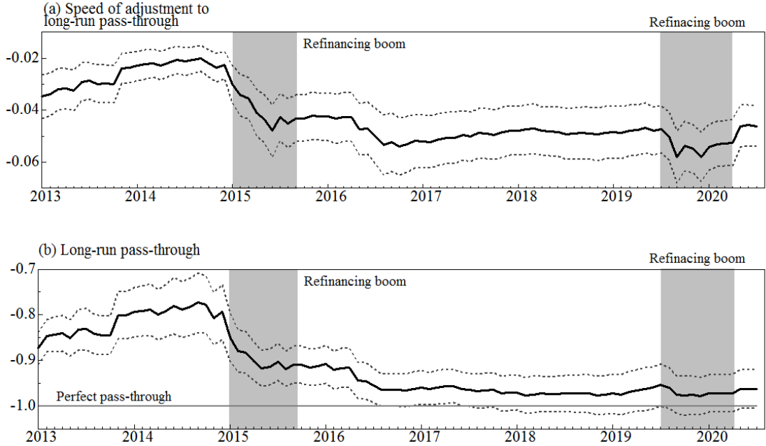
Figure 12: Rolling-window estimation
