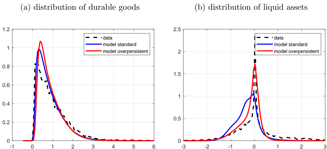
Figure 7: Model Fit
