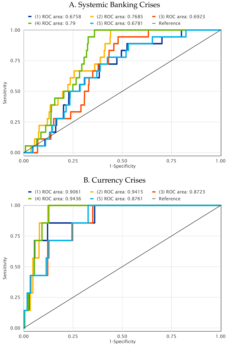
Figure 9: Comparison of ROC curves for each model
