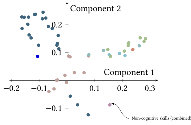
Figure 15: Loading plot
