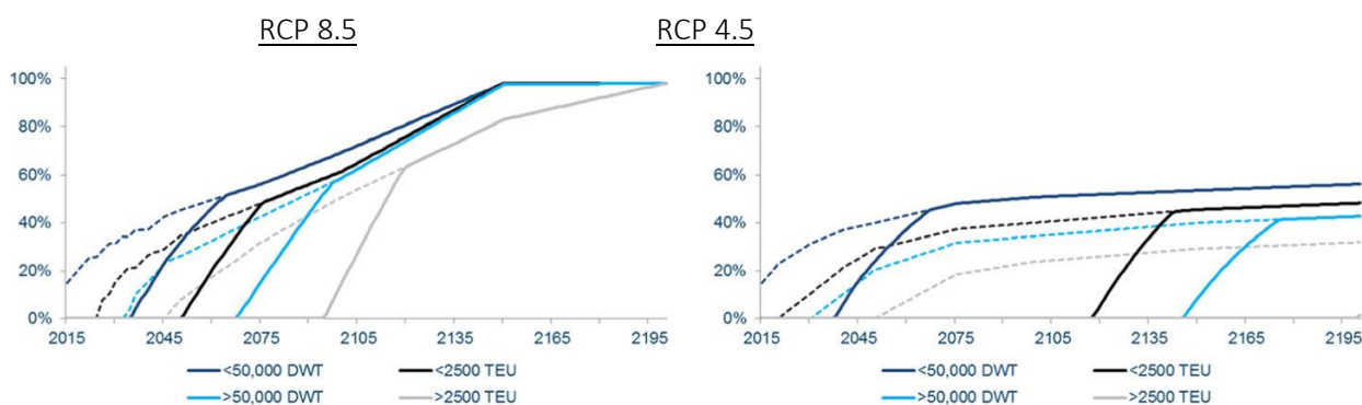
Figure 6. Norther Sea Route re-routing of four ship categories under RCP 8.5 and RCP 4.5
