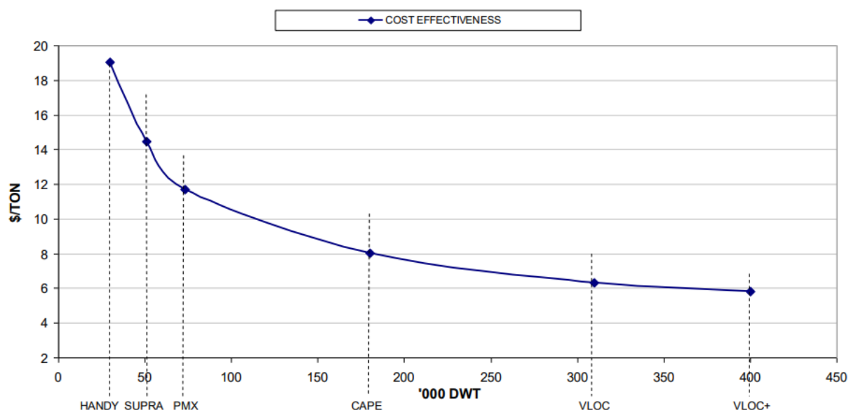
Figure 7. Cost-effectiveness of different size bulk carriers carrying ore from Australia to China
