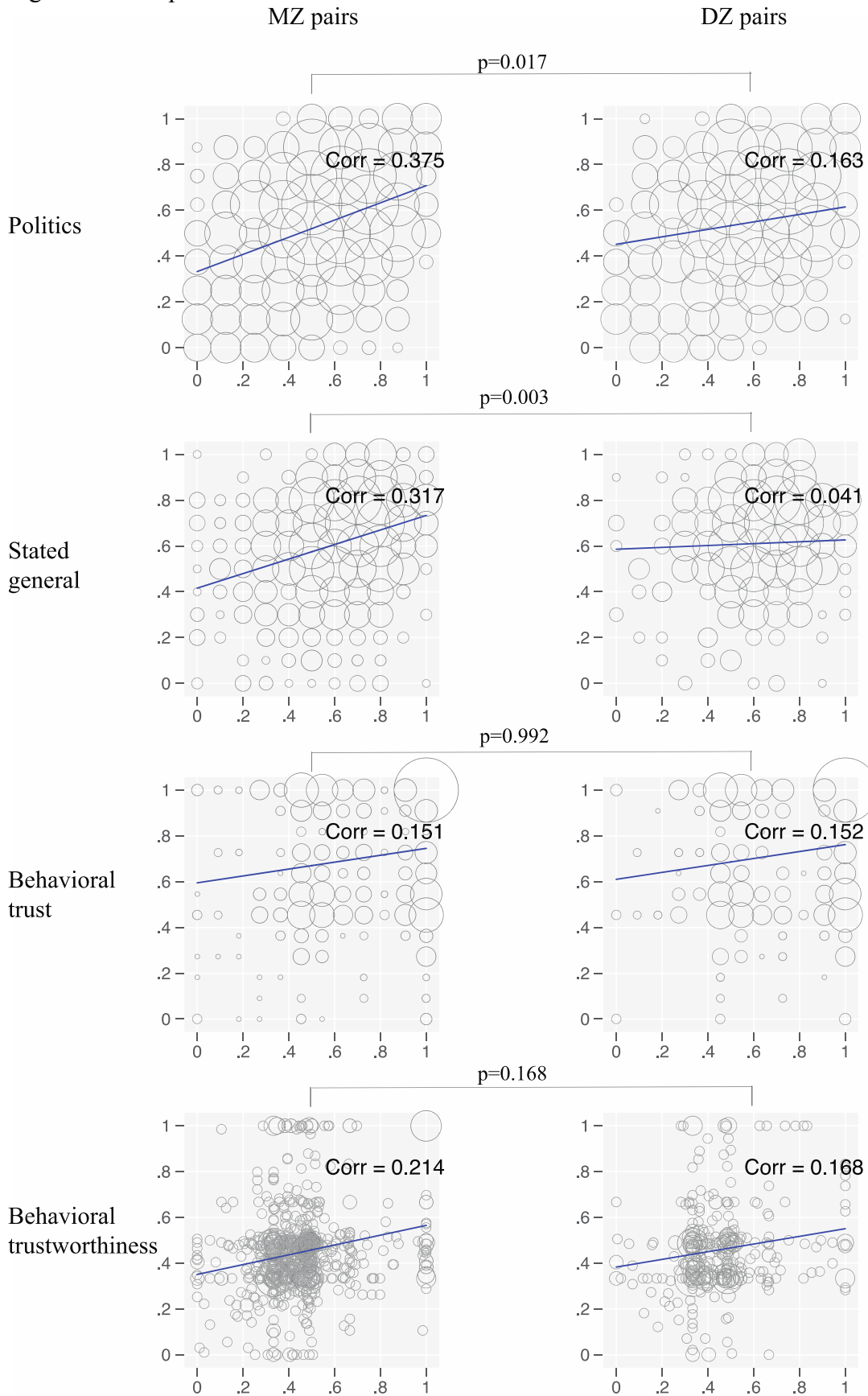
Figure 1: Twin pair trust correlations
