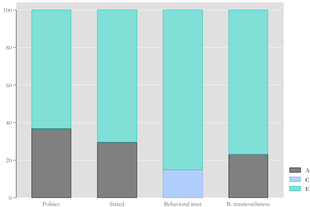
Figure 2: Proportion of variance explained by additive genes and environment.
