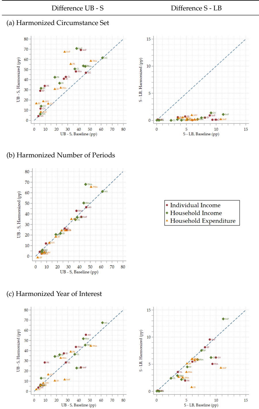
Figure 3: Sensitivity Checks
