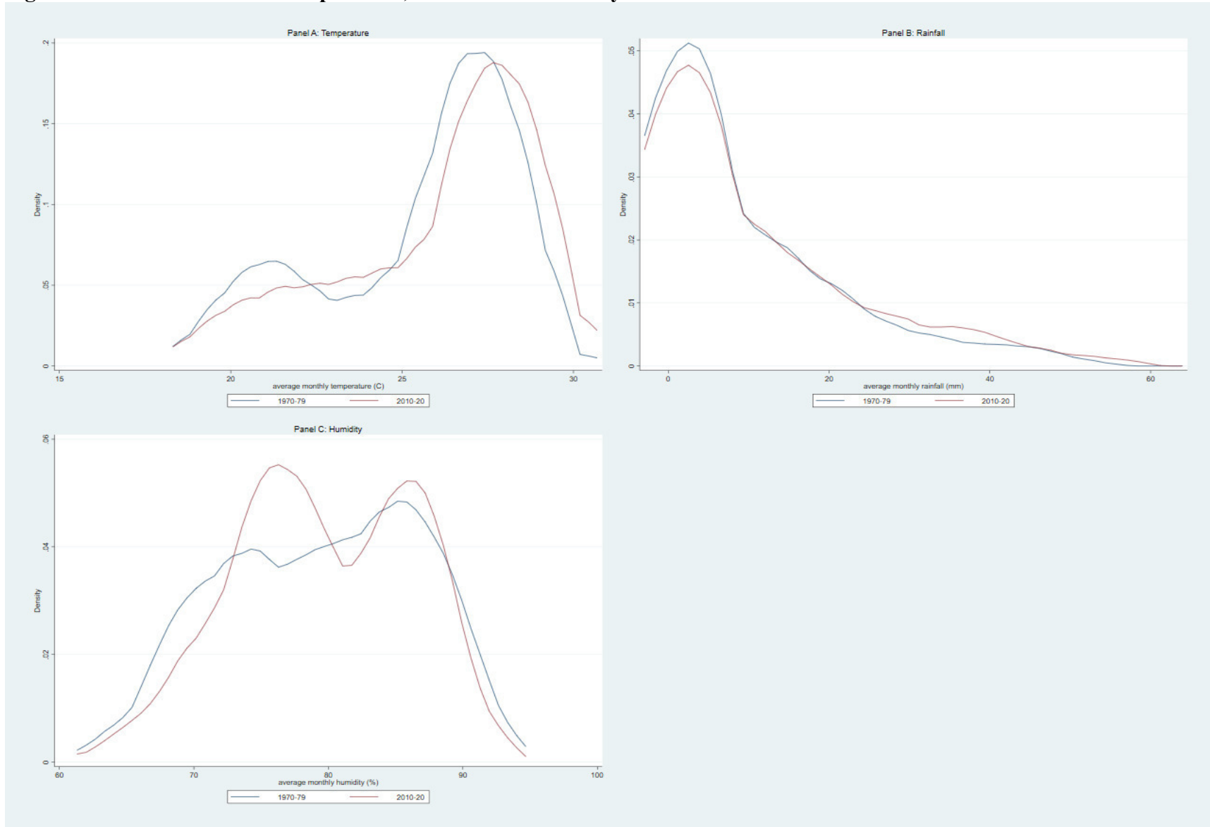
Figure 3: Kernel densities of temperature, rainfall and humidity 1970-2020
