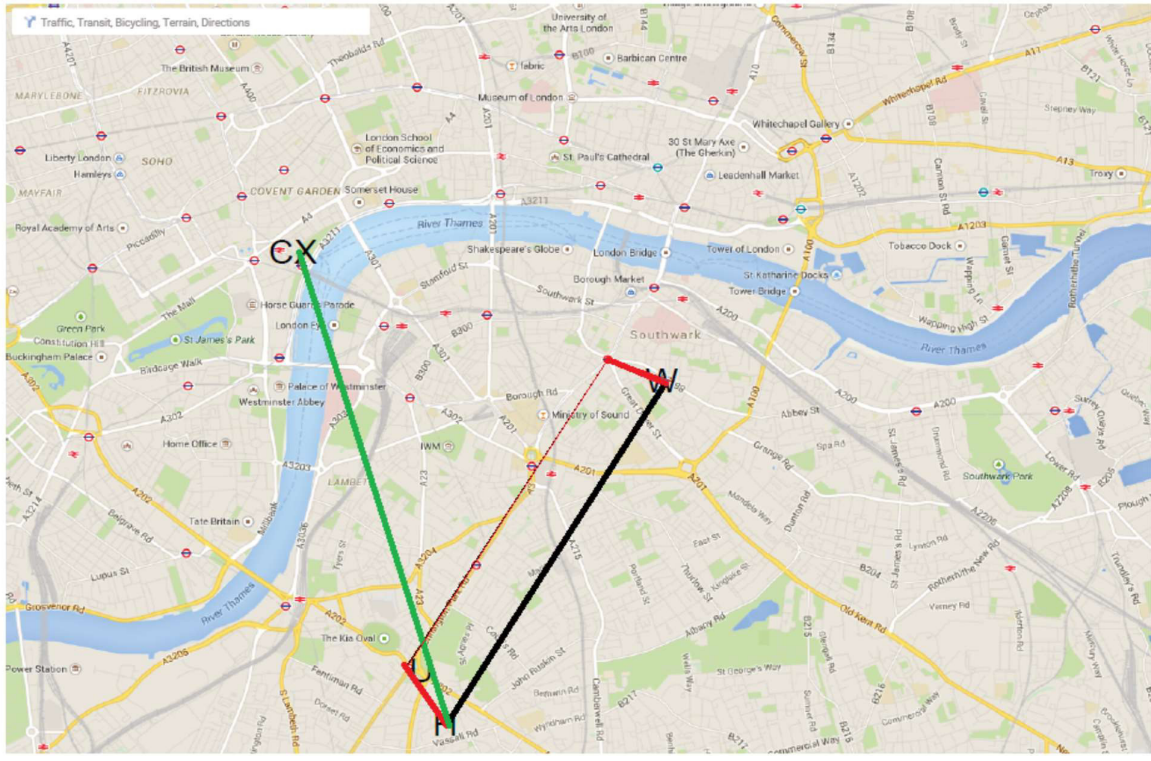
Figure A.II.1 Distances for One Individual
