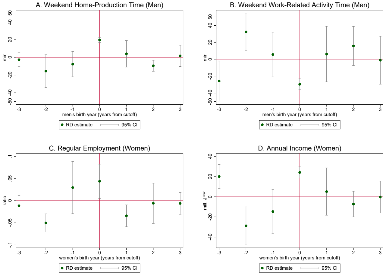
Figure 6: Results of Placebo Test
