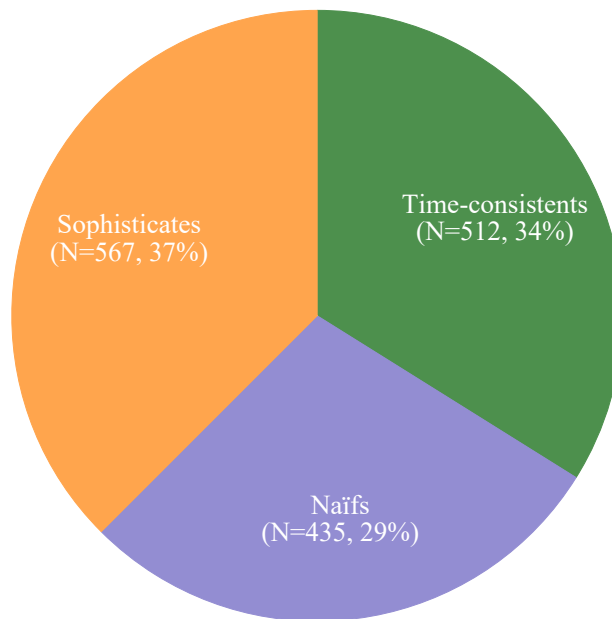
Figure 3: Type distribution
