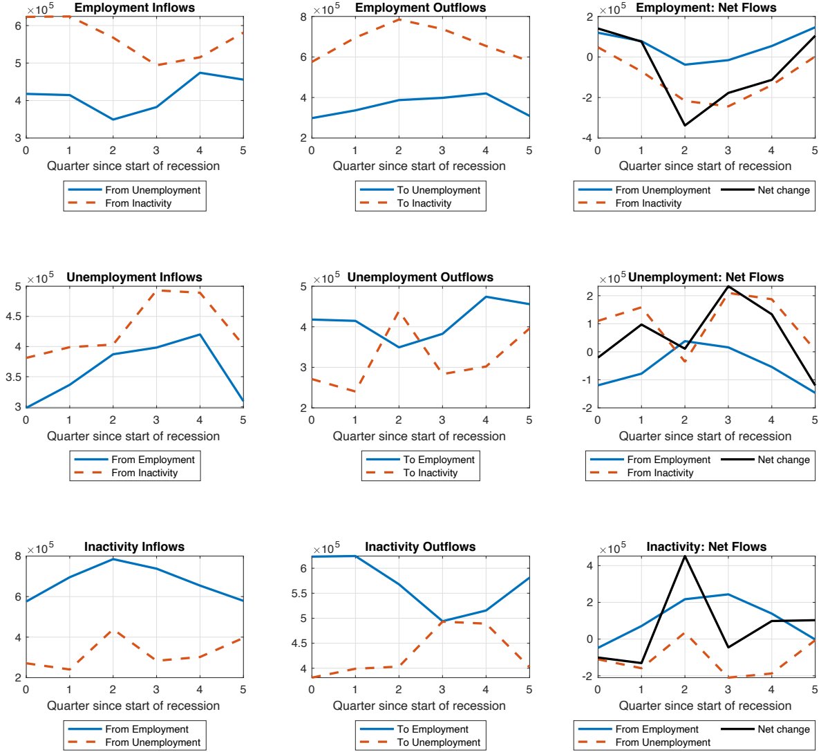
Figure 2: Aggregate Labour Market Flows during Covid-19
