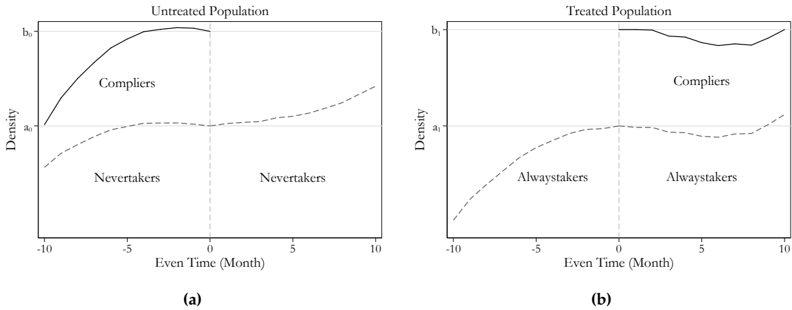
Figure 8: Selection Analysis.
