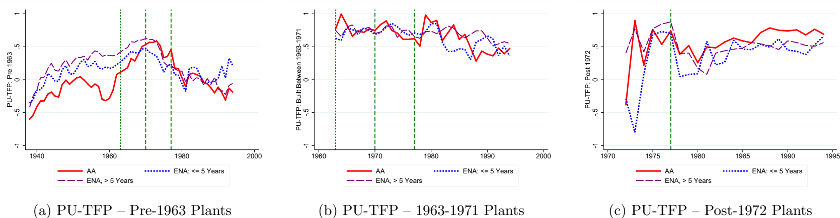
Figure C.7: Annual Average Total Factor Productivity from Fossil-Fuel Power Plants by Vintage and Years in Nonattainment
