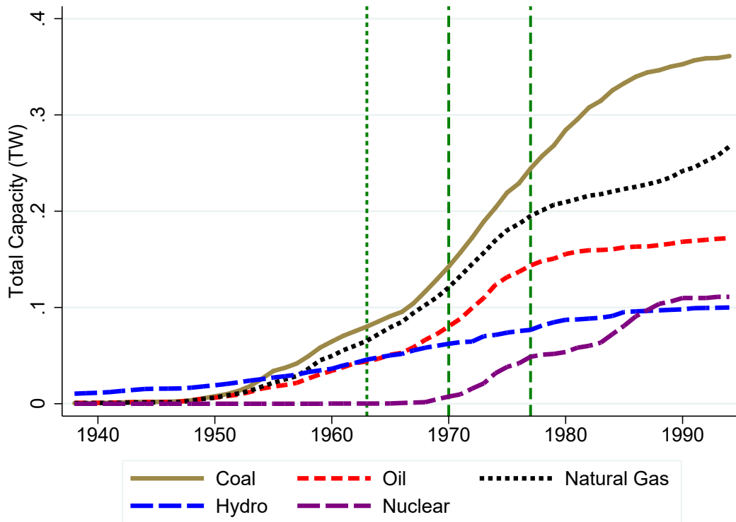
Figure C.4: Annual Total Electricity Generating Capacity by Fuel Type
