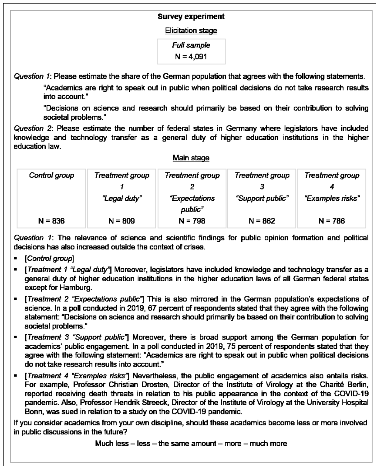
Figure 1: Experimental design
