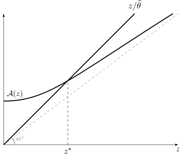
Figure 1: Determination of the cutoff productivity z^*
