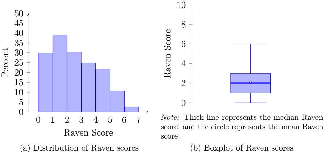
Figure 1: Raven scores
