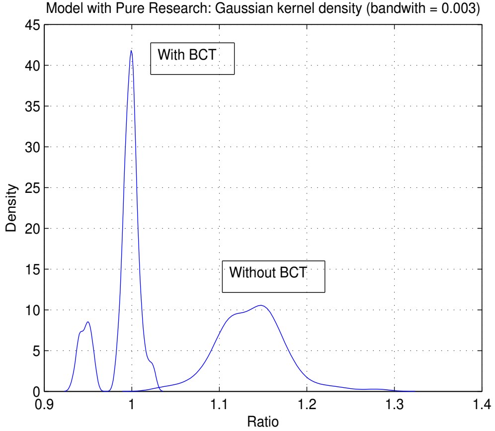
Figure 5: Distribution of the employment ratio (kernel density estimation).
