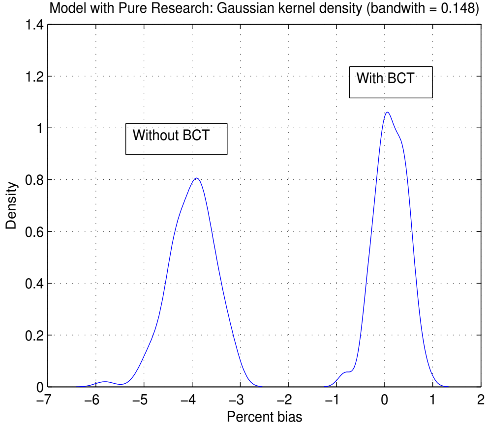
Figure 4: Distribution of the percent forecast error (kernel density estimation).
