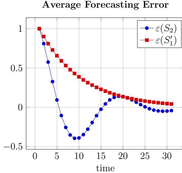
Figure 2: Average Forecasting Error without BC (system S'_1; \alpha = 0.9 ) and with incomplete BC (system S_2; \alpha = \gamma = 0.9 )
