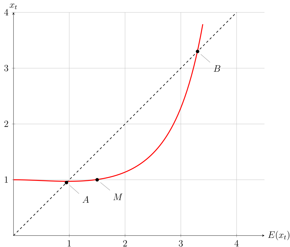
Figure 7: Model consistent expectations and unbiased solutions
