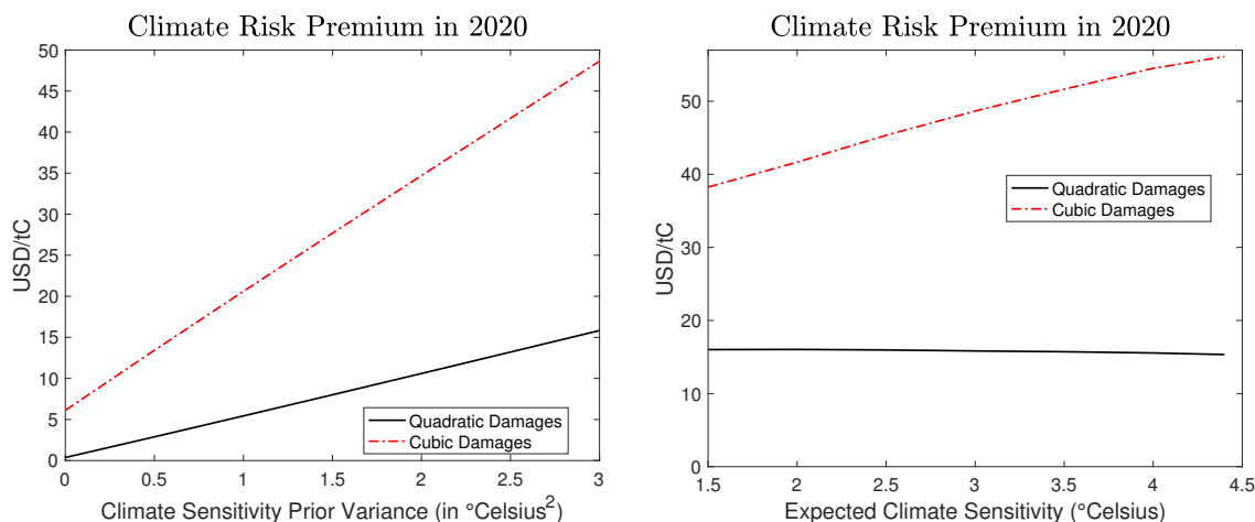
Figure 4: Dependence of the SCC’s risk premium in 2020 on the prior’s variance (left) and the expected climate sensitivity (right).
