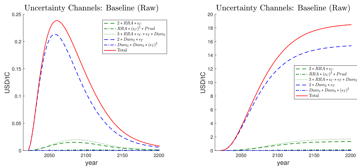
Figure 2: Contributions of climate sensitivity uncertainty to the SCC based on Proposition 2 for our baseline calibration of DICE 2013. The left panel shows the contributions to the SCC in 2020 from a given year in the future, whereas the right panel shows the cumulative contributions corresponding to the depicted time horizon.
