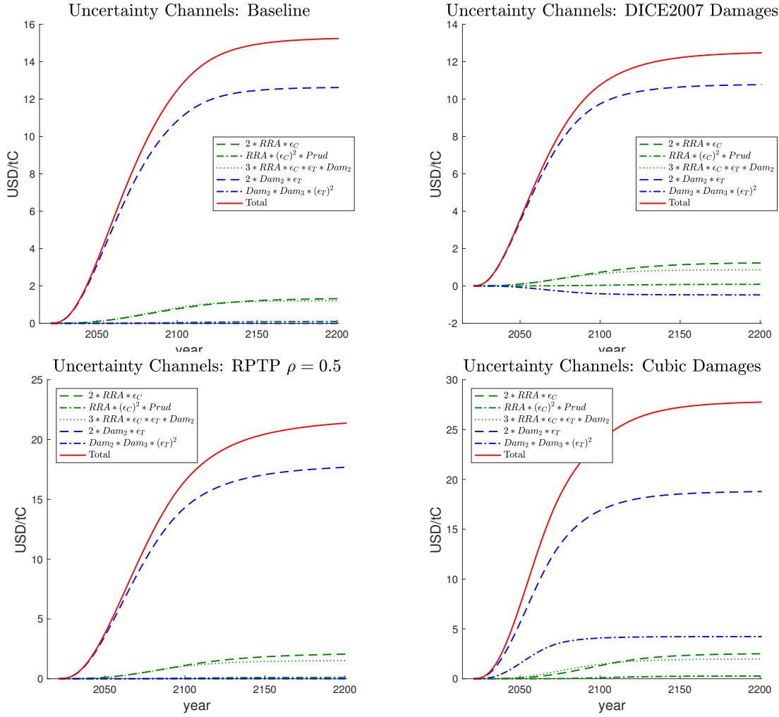
Figure 5: Uncertainty about climate sensitivity. Cumulative contribution to the SCC's risk premium in 2020 by channel for different scenarios.
