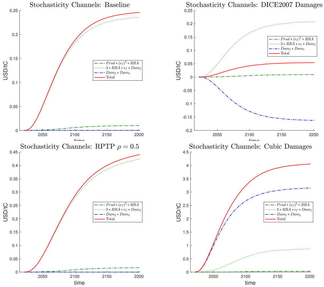
Figure 6: Stochastic temperature evolution. Cumulative contribution to the SCC's risk premium in 2020 by channel for different scenarios.
