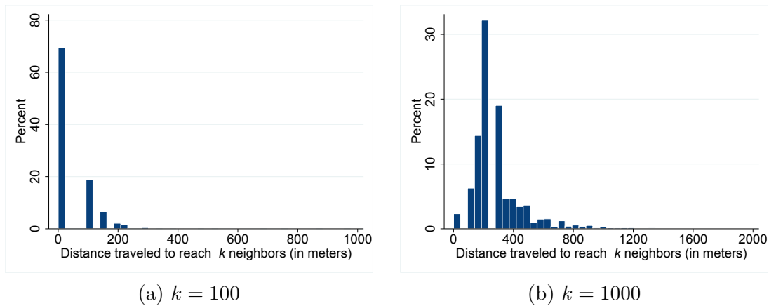
Figure A.2: Distance traveled by EquiPop software to find k neighbors
