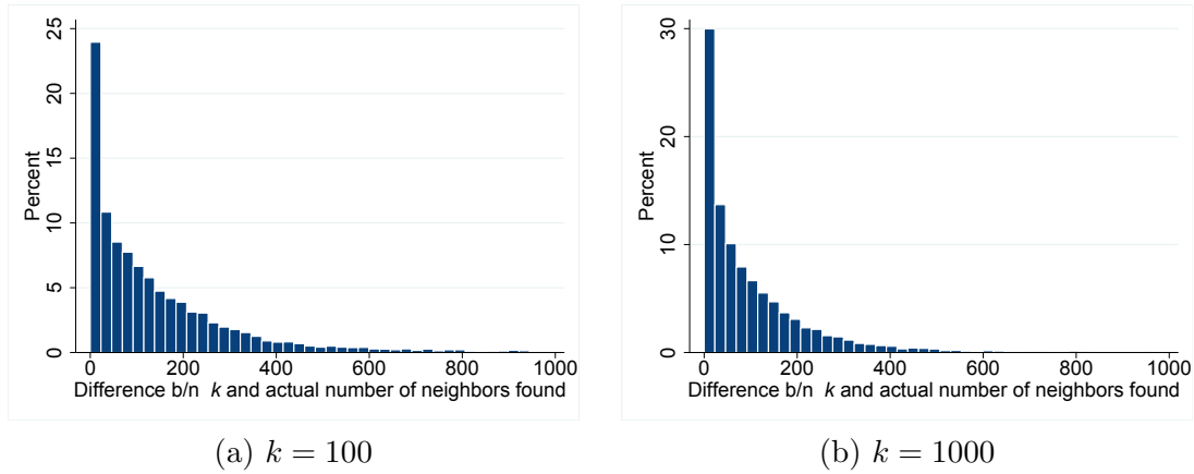
Figure A.1: Difference between k and observed k
