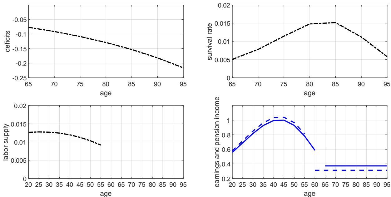
Figure 2: Blue-Collar Life-Cycle Outcomes: Status Quo vs. Fair Pension with Early Retirement
