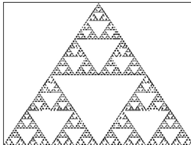
Figure 2. Sierpinski triangle.
