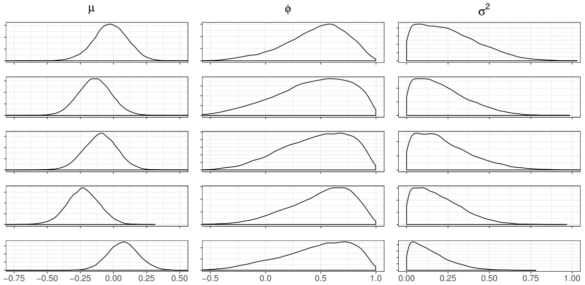
Figure 23 Posterior distributions of volatility parameters, normally distributed data
