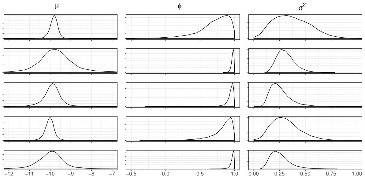
Figure 24 Posterior distributions of volatility parameters, normally distributed data with stochastic volatility
