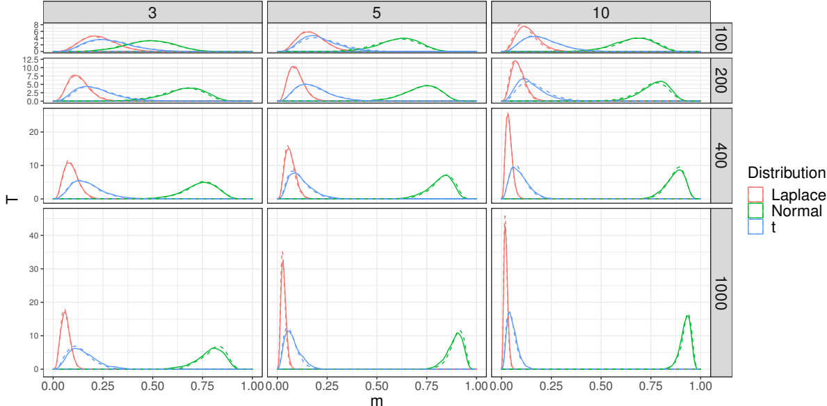
Figure 16 Posterior distributions of the weights, normally distributed data
