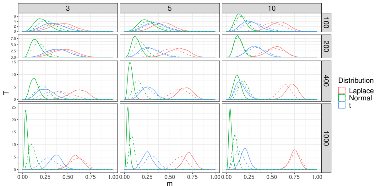
Figure 20 Posterior distributions of the weights, Laplace distributed data with stochastic volatility
