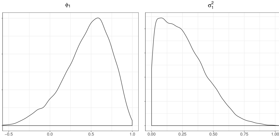
Figure 4 Posterior distributions of volatility parameters \phi_1 and \check{\sigma}_1^2 , normally distributed data, m = 5 and T = 200
