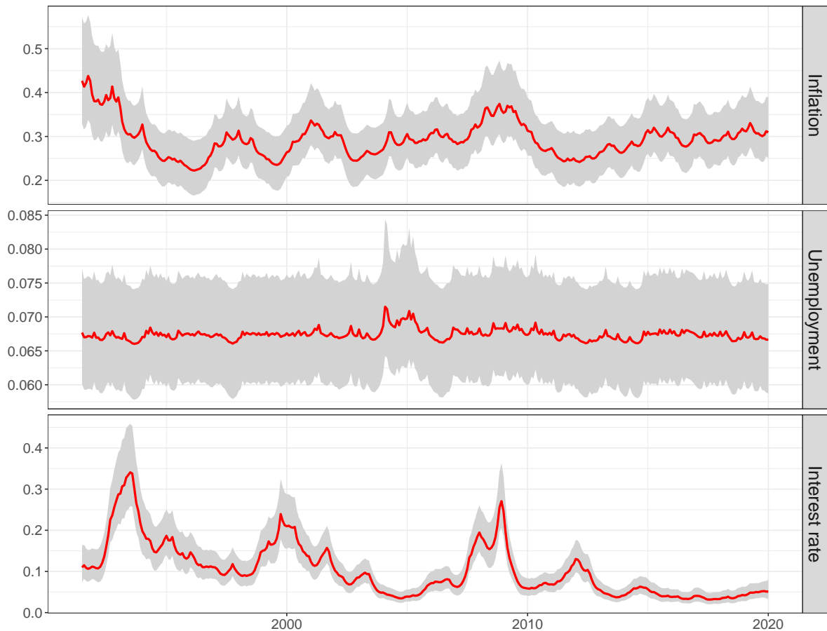
Figure 10 Posterior distribution of volatilities, small VAR - Germany
