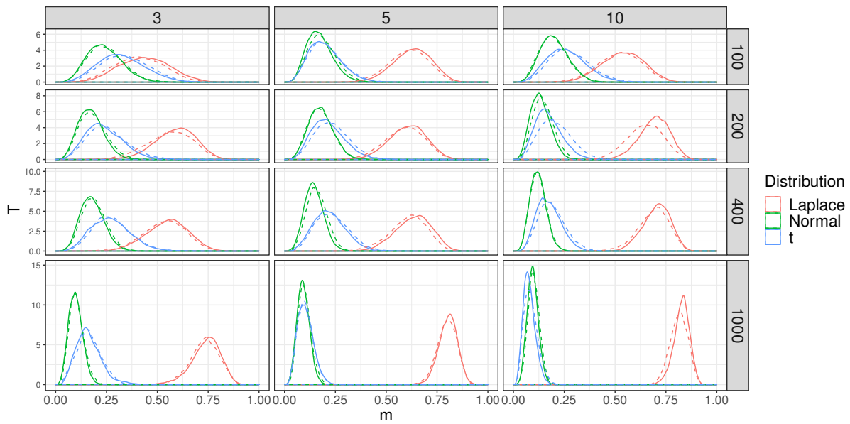
Figure 19 Posterior distributions of the weights, Laplace distributed data
