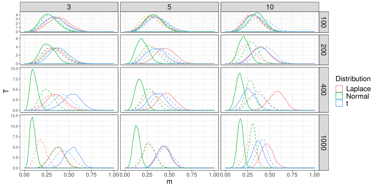
Figure 22 Posterior distributions of the weights, mixture distributed data with stochastic volatility
