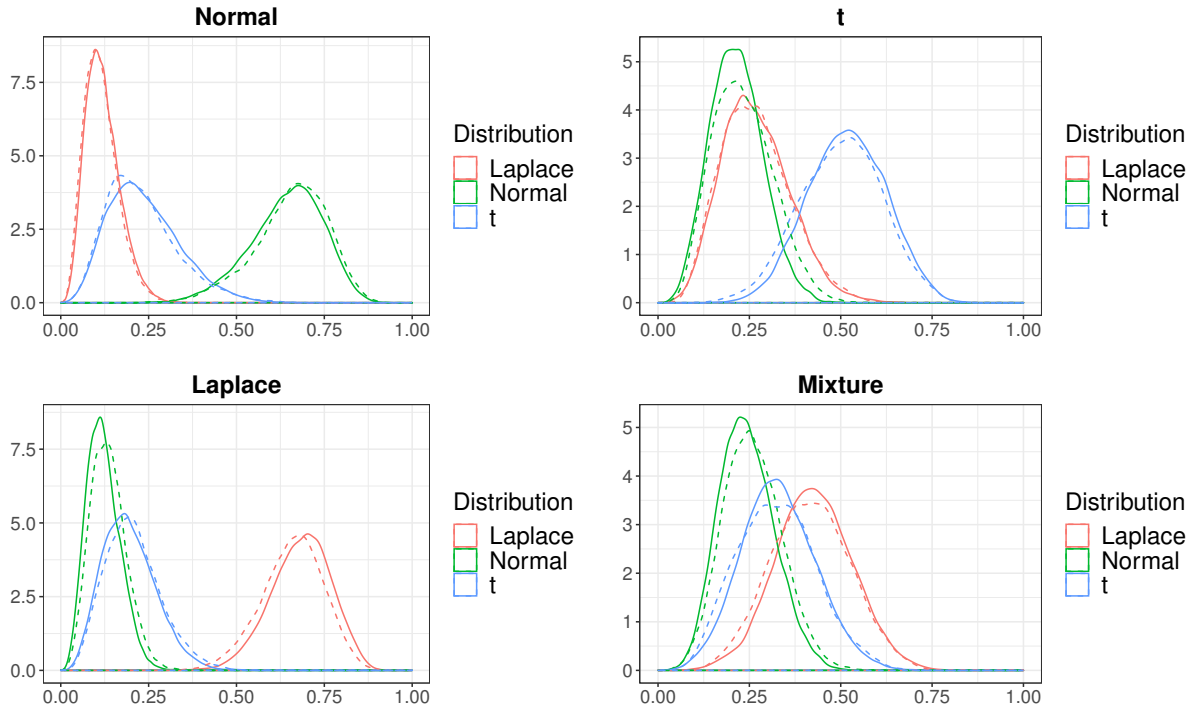
Figure 2 Posterior distributions of the weights, simulated data, m = 5 and T = 200
