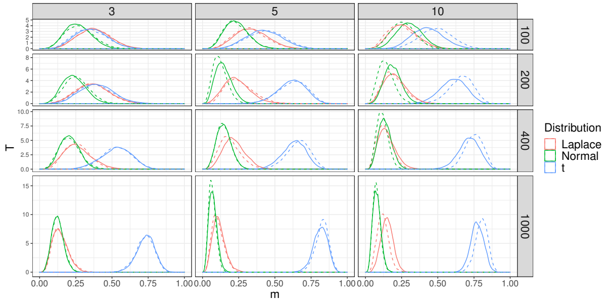
Figure 18 Posterior distributions of the weights, t -distributed data with 3 degrees of freedom
