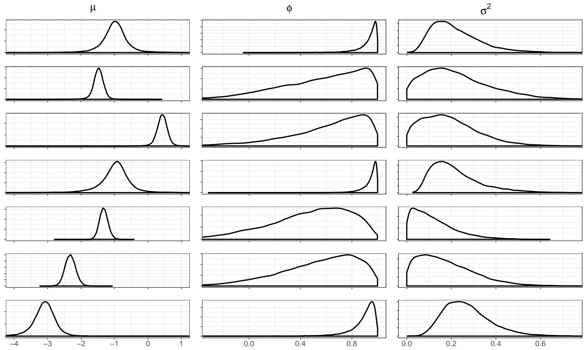
Figure 13 Posterior distribution of volatility parameters, medium VAR
