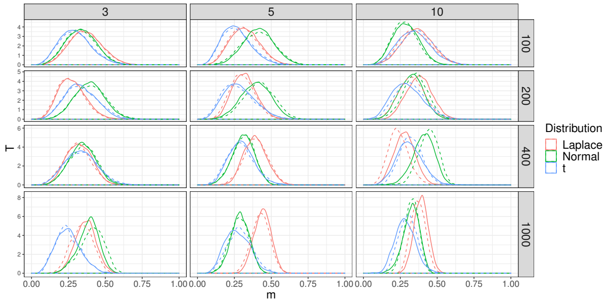
Figure 21 Posterior distributions of the weights, mixture distributed data
