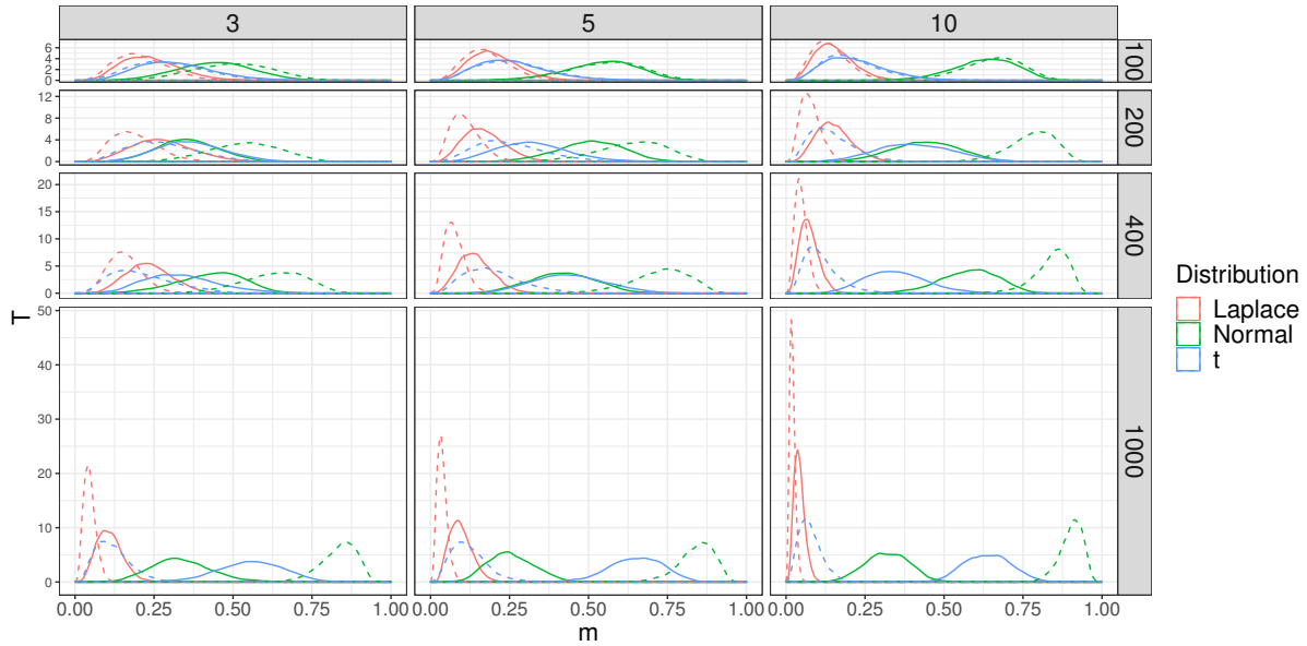
Figure 17 Posterior distributions of the weights, normally distributed data with stochastic volatility
