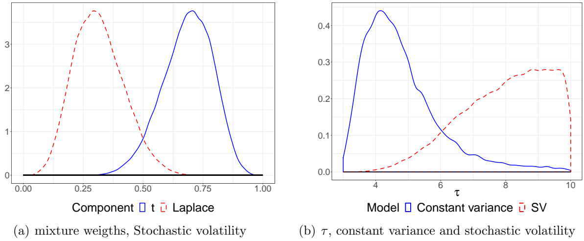
Figure 8 Posterior distribution of mixture parameters, small VAR - Germany
