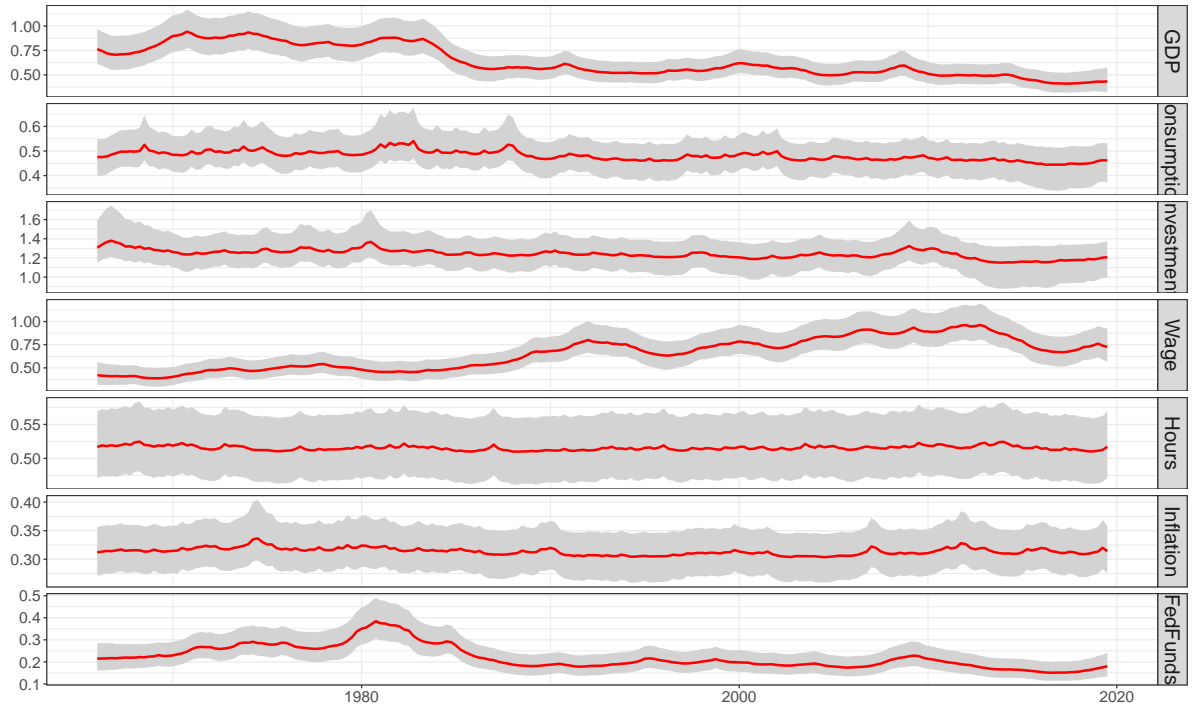
Figure 14 Posterior distribution of volatilities, medium VAR
