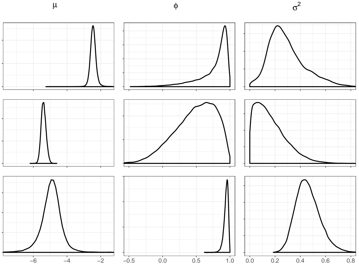
Figure 9 Posterior distribution of volatility parameters, small VAR - Germany
