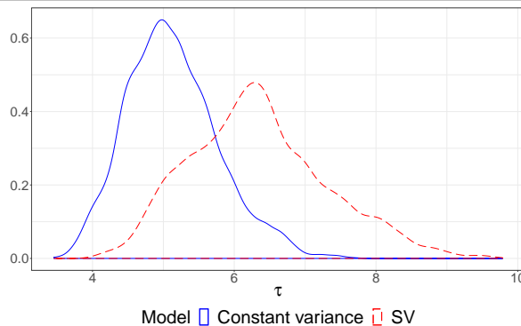
Figure 15 Posterior distribution for \tau , constant variance and stochastic volatility, medium VAR
