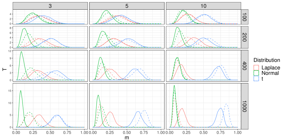
Figure 3 Posterior distributions of the weights, t -distributed data with 3 degrees of freedom and stochastic volatility
