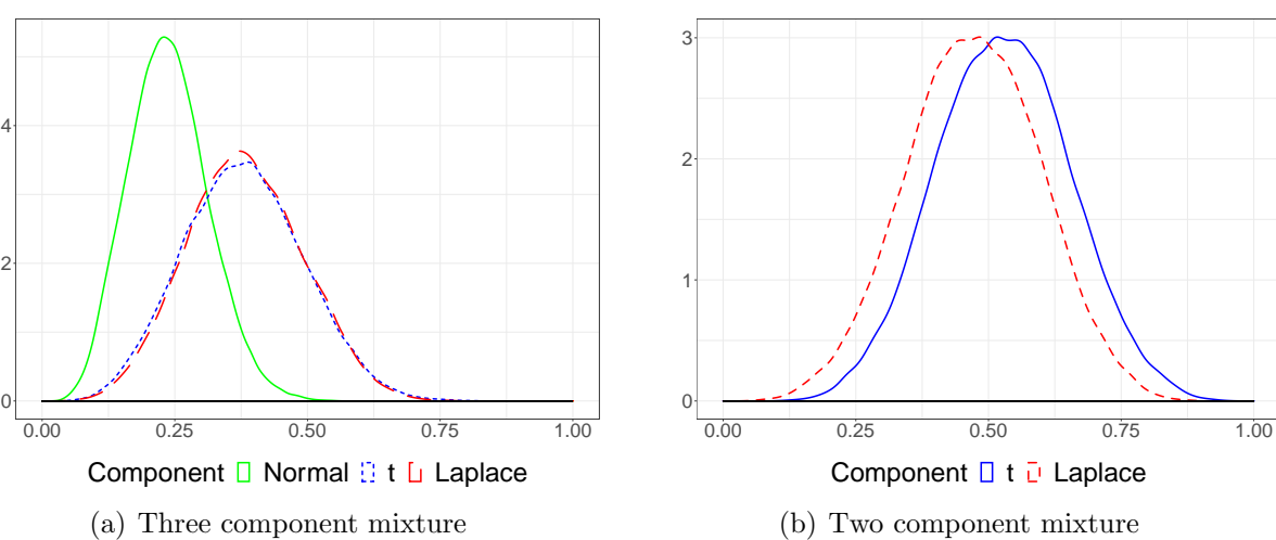
Figure 7 Posterior distribution of mixture weights, small VAR - Germany
