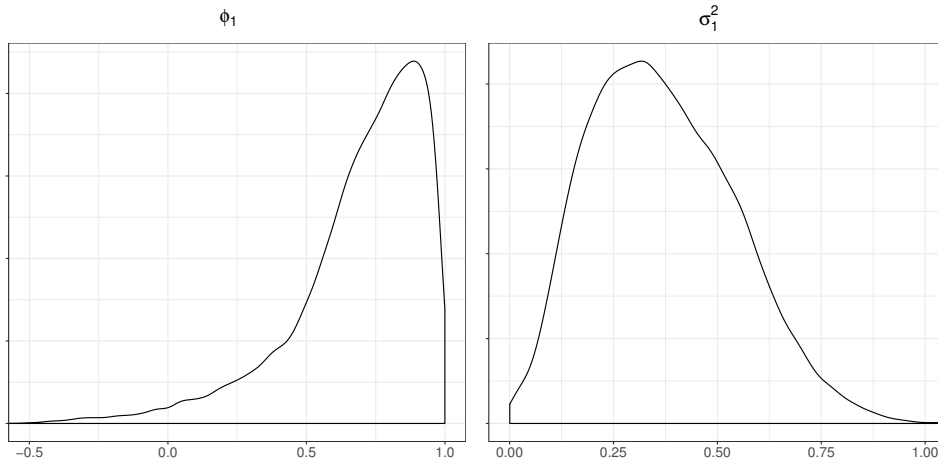
Figure 5 Posterior distributions of volatility parameters \phi_1 and \check{\sigma}_1^2 , normally distributed data with stochastic volatility, m = 5 and T = 200
