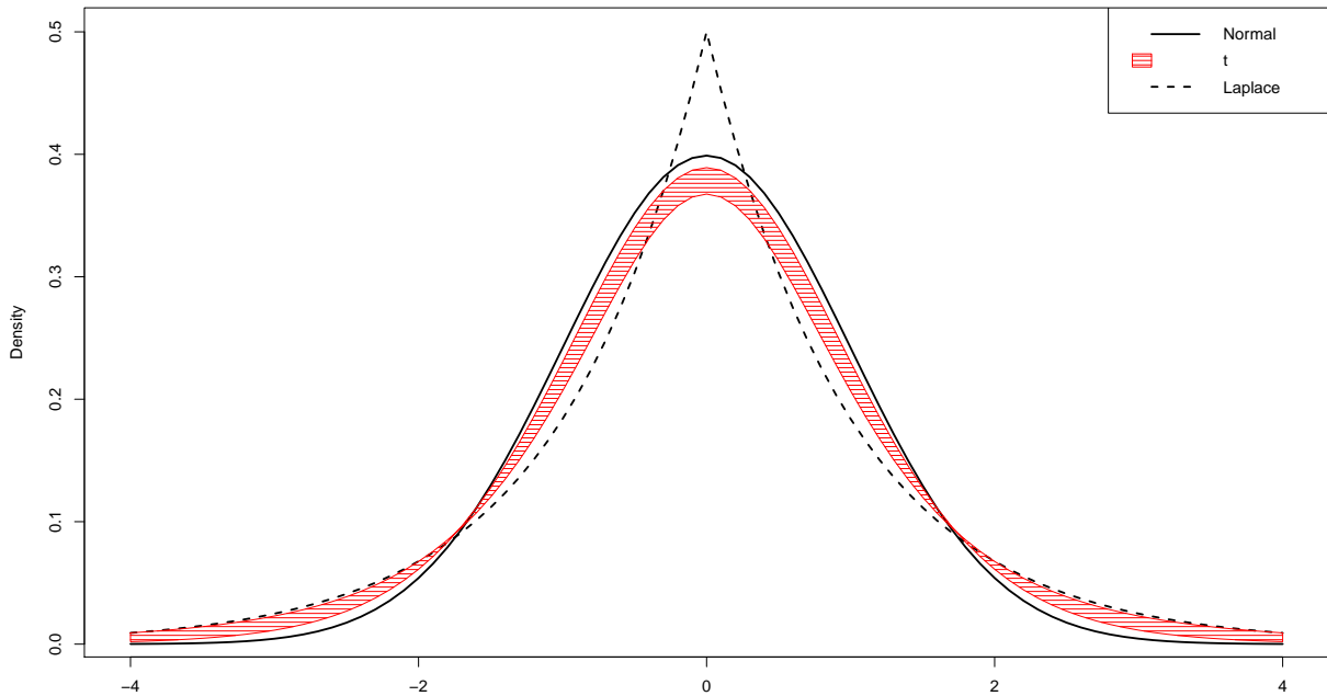
Figure 1 Distributional shapes covered by the mixture
