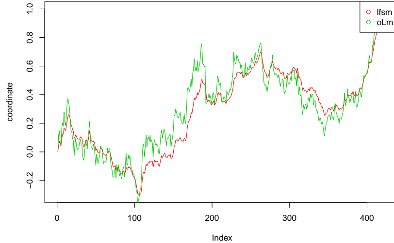
Figure 6: Plot of sample path and Lévy motion with seed=2
