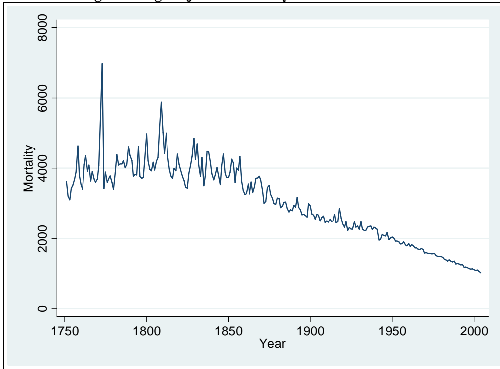
Figure 1: Age adjusted mortality in Sweden 1751-2004
