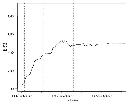
Figure 6: Squared bias ratio, proportion Yes
