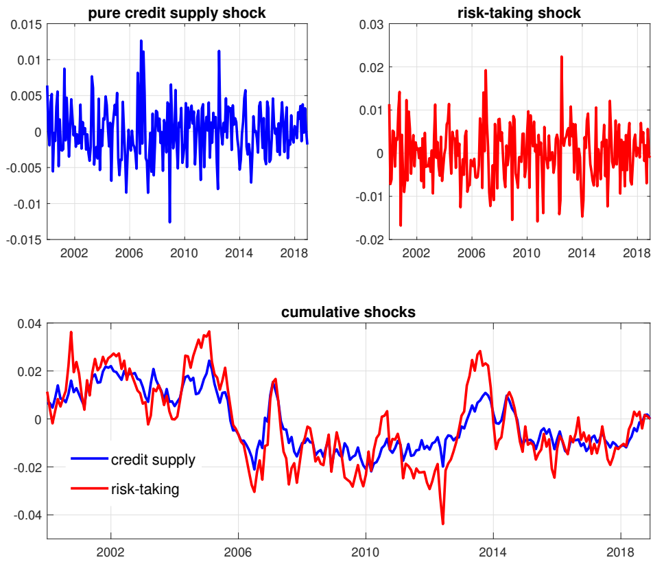
Figure 7: Decomposed shock series
