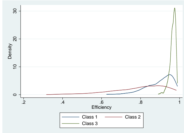
Figure 1: Kernel density estimates of cost efficiency
