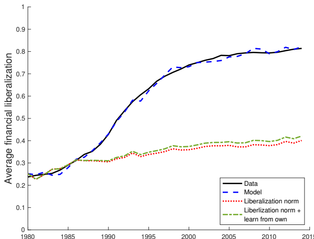
Figure 20: Decomposition of the estimated model with common- \beta growth specification
