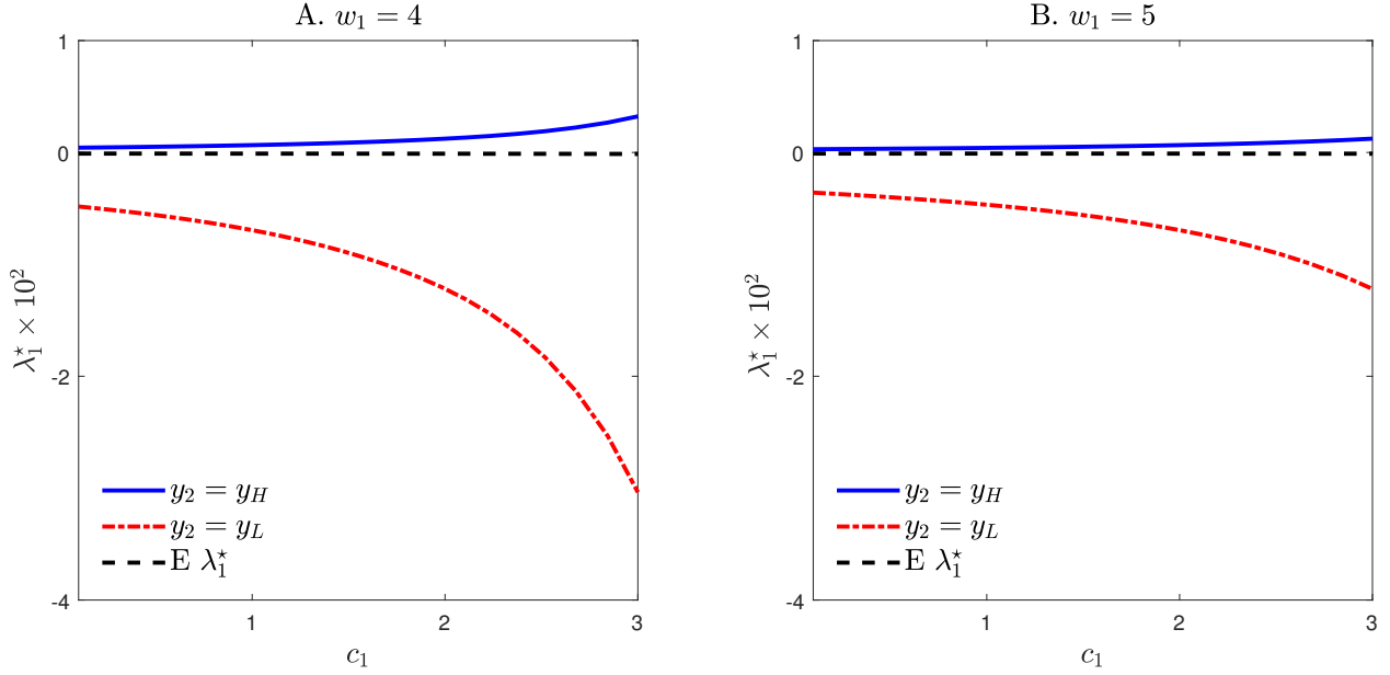
Figure 1: Ideal penalty. The ideal penalty \lambda_1^* for the consumption-saving problem of Section 2, plotted as a function of time-1 consumption choice c_1 . We use the parameters shown in Table 1. The agent believes the probability of y_H is 0.89. Panel A corresponds to the time-1 wealth w_1 = 4 , while Panel B corresponds to w_1 = 5 . The solid line is the penalty function in the state y_2 = y_H , while the dash-dot line is the penalty in the state y_2 = y_L . The dash line shows the expected value of the penalty over the two possible realizations of y_2 . This expectation is identically equal to zero.
