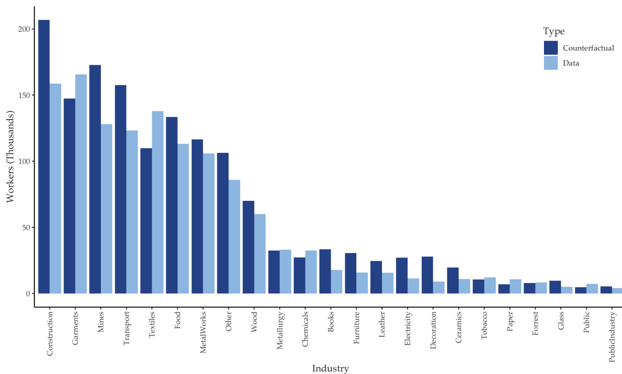
Figure 11: No WWI Cf: Sectoral Employment (1920 Data vs Cf)
