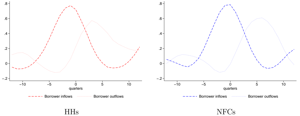
Figure 13: Cross-correlations
